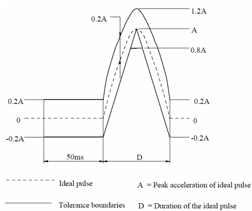
Figure 2 Pulse Shape (Half Sine)
